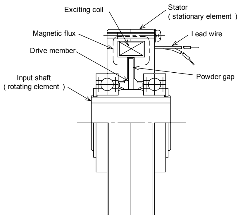
Fig. 1 ZX-YN powder brakes (representative examples)
