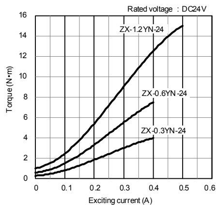
Fig.2 Exciting current v.s. torque characteristics (representative examples)
